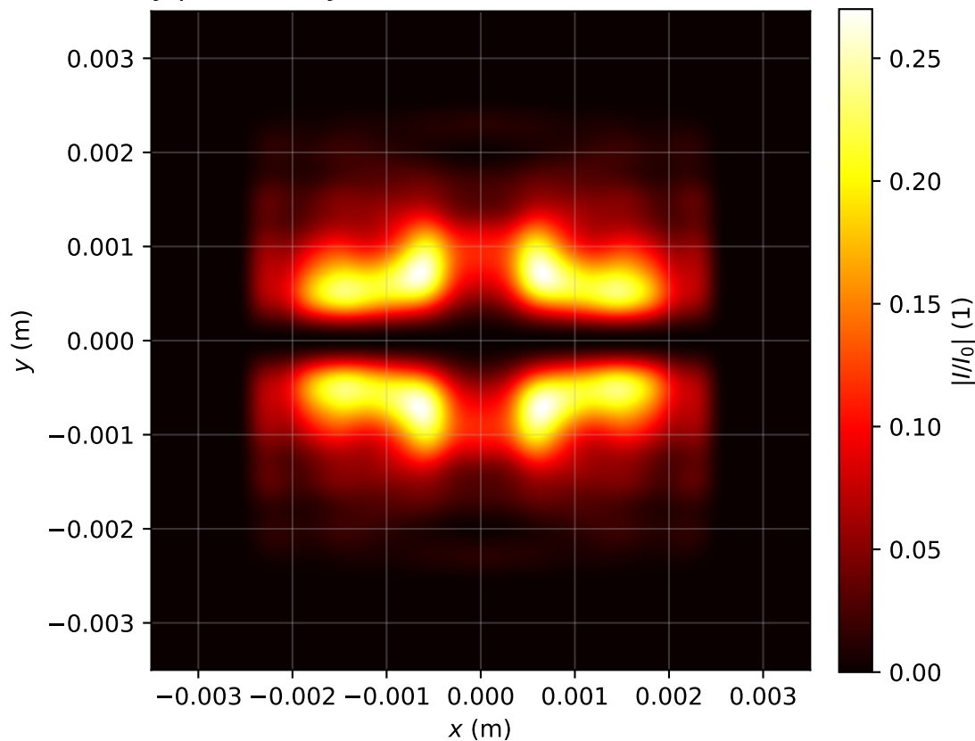
Intensity profile I(x, y, z = 3.662)/I_0 , \text{Pin}=4.0\text{Pcr} , artificial time
